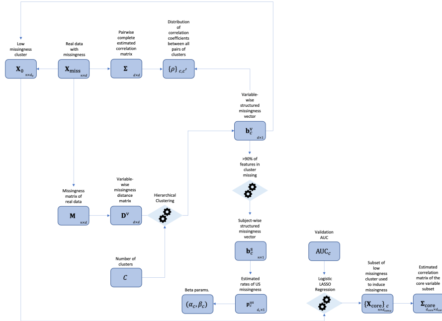
Figure 1: Flow chart of the data analysis pipeline.
