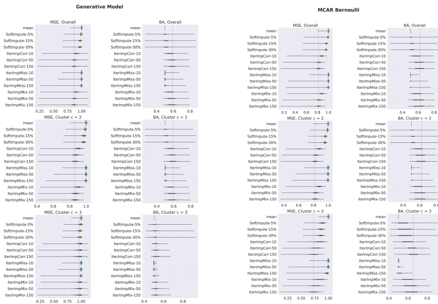
Figure 7: Violin plots of the imputation accuracy by variable. The red line in each violin plot is the median of the best performing method in that comparison, i.e., the lowest median MSE and the highest median BA. Since continuous data is standardised, the MSE scores correspond to 1 minus the variance explained by prediction. It is obvious that iterative imputation that uses Pearson correlation as its criterion for selecting k variables is the best performing method overall. It is also notable that SoftImpute performs poorly for binary data. When comparing the performance between generative model versus completely unstructured missing data, we can see that performance is better for the completely unstructured case, for both continuous and binary variables. This difference is particularly stark for cluster c = 3 , where there is a lot of structured missingness and very little unstructured missingness, highlighting the difficulty of imputation in this setting.
