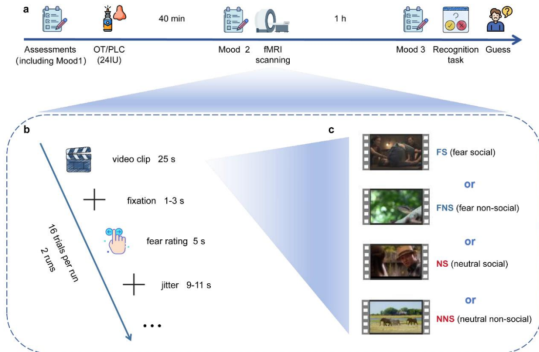
Fig. 1 Experimental timeline, paradigm and schematic depiction of stimuli. a The timeline of the whole experiment. b Naturalistic fear induction and rating paradigm. c Example stimuli. In each run, 4 types of video clips were presented (FS, FNS, NS, NNS) according to a randomized order. Abbreviations: OT oxytocin, PLC placebo, fMRI functional magnetic resonance imaging, FS fear social, FNS fear non-social, NS neutral social, NNS neutral non-social. License: Images in 1a and 1b were obtained from Flaticon.com under the free license with attribution.
