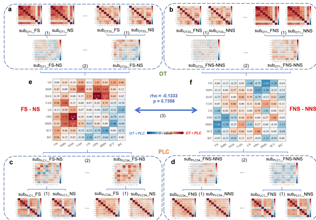
Fig. 4 OT enhanced functional connectivity on the level of large-scale networks. a b c d Flow of z-value matrix calculation for the degree of response functional connectivity under specific contrasts. (1) The Fisher r-z matrices of each condition for each participant were subtracted to yield a new matrix of z-value corresponding to the contrast (e.g. z_{FS} - z_{NS} = z_{FS} - z_{NS} ). (2) New matrices of z-value corresponding to a specific contrast were generated for each participant in each group, which were used as features in a two-sample t-test to derive the between-group differences under the specified contrast. e OT significantly strengthened the functional connectivity between FPN and DAN as well as DMN and DAN in the fear social-related contrast f but not in the fear non-social-related contrast. OT oxytocin, PLC placebo, FS fear social, FNS fear non-social, NS neutral social, NNS neutral non-social, VN visual network, SMN somatomotor network, DAN dorsal attention network, VAN ventral attention network, LN limbic network, FPN frontoparietal network, DMN default mode network, SCT subcortical network, B/C brainstem and cerebellum. ## p_{\text{un-corrected}} < 0.01 , # p_{\text{un-corrected}} < 0.05 .
