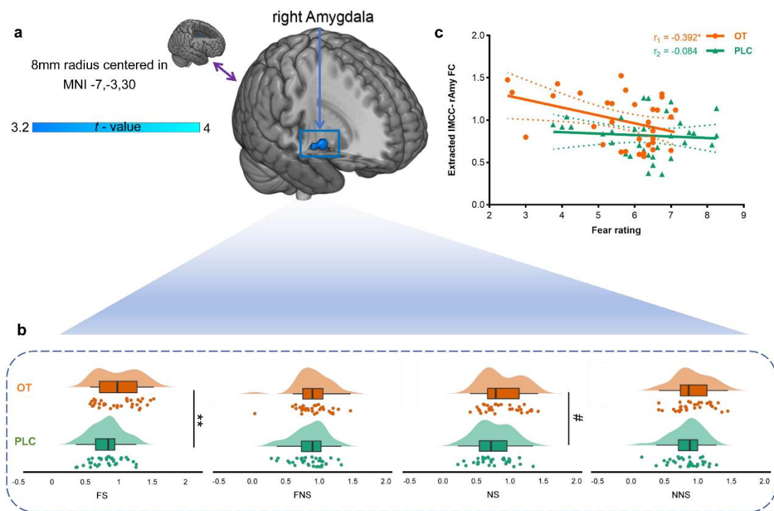
Fig. 3 OT strengthened IMCC-rAmy communication specifically in social fear contexts. a Interaction effect between treatment \times emotion \times social on IMCC connectivity with the right amygdala b OT specifically increased functional connectivity between IMCC and rAmy in the FS contexts but not other conditions and c The functional connectivity between IMCC and rAmy was significantly negatively correlated with subjective fear experience in OT group but not PLC group. OT oxytocin, PLC placebo, FS fear social, FNS fear non-social, NS neutral social, NNS neutral non-social. ** p_{\text{FDR-corrected}} < 0.01 , * p_{\text{FDR-corrected}} < 0.05 , # p_{\text{uncorrected}} < 0.05 .
