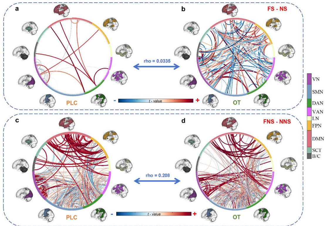
Fig. 5 Comparison between treatment groups for whole-brain functional connectivity during social and non-social fear separately. Under fear social contexts, a PLC group showed a sparse connectivity between brain regions b the OT group exhibited stronger functional interactions at the whole-brain level. In contrast, under the fear non-social context c PLC and d OT groups showed similar whole-brain functional connectivity patterns. OT oxytocin, PLC placebo, FS fear social, FNS fear non-social, NS neutral social, NNS neutral non-social, VN visual network, SMN somatomotor network, DAN dorsal attention network, VAN ventral attention network, LN limbic network, FPN frontoparietal network, DMN default mode network, SCT subcortical network, B/C brainstem and cerebellum.
