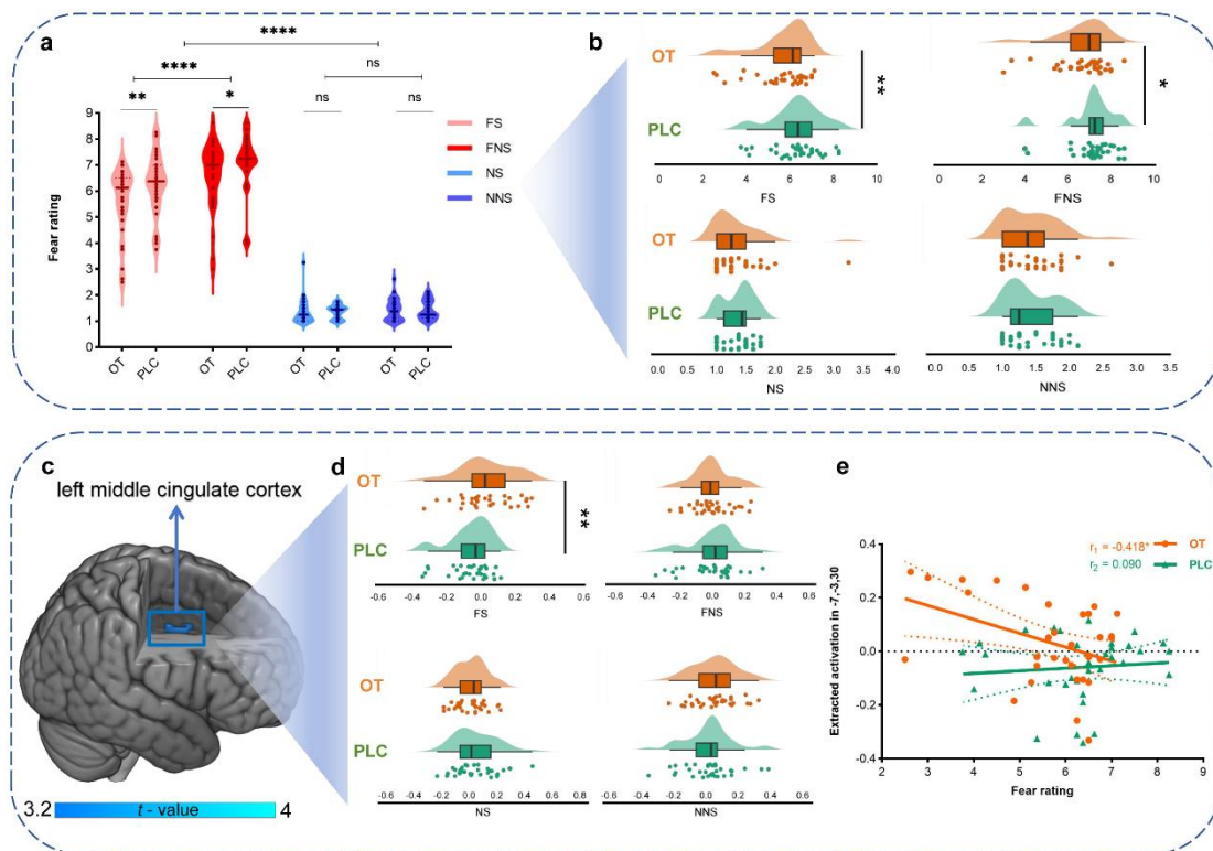
Fig. 2 The effects of OT on behavioral fear rating and cingulate activity. a OT reduced subjective fear rating in naturalistic situations particularly in contexts, b OT effects on fear rating under four conditions separately, c OT but not PLC could strengthen the activation in the left middle cingulate cortex (IMCC) under the interaction of valence and social. Particularly, d OT specifically increased the activation in IMCC under FS but not other conditions. e The activation in IMCC was significantly negatively correlated with subjective fear experience in OT group but not PLC group. OT oxytocin, PLC placebo, FS fear social, FNS fear non-social, NS neutral social, NNS neutral non-social. **** p_{\text{FDR-corrected}} < 0.0001 , *** p_{\text{FDR-corrected}} < 0.001 , ** p_{\text{FDR-corrected}} < 0.01 , * p_{\text{FDR-corrected}} < 0.05 , ns not significant.
