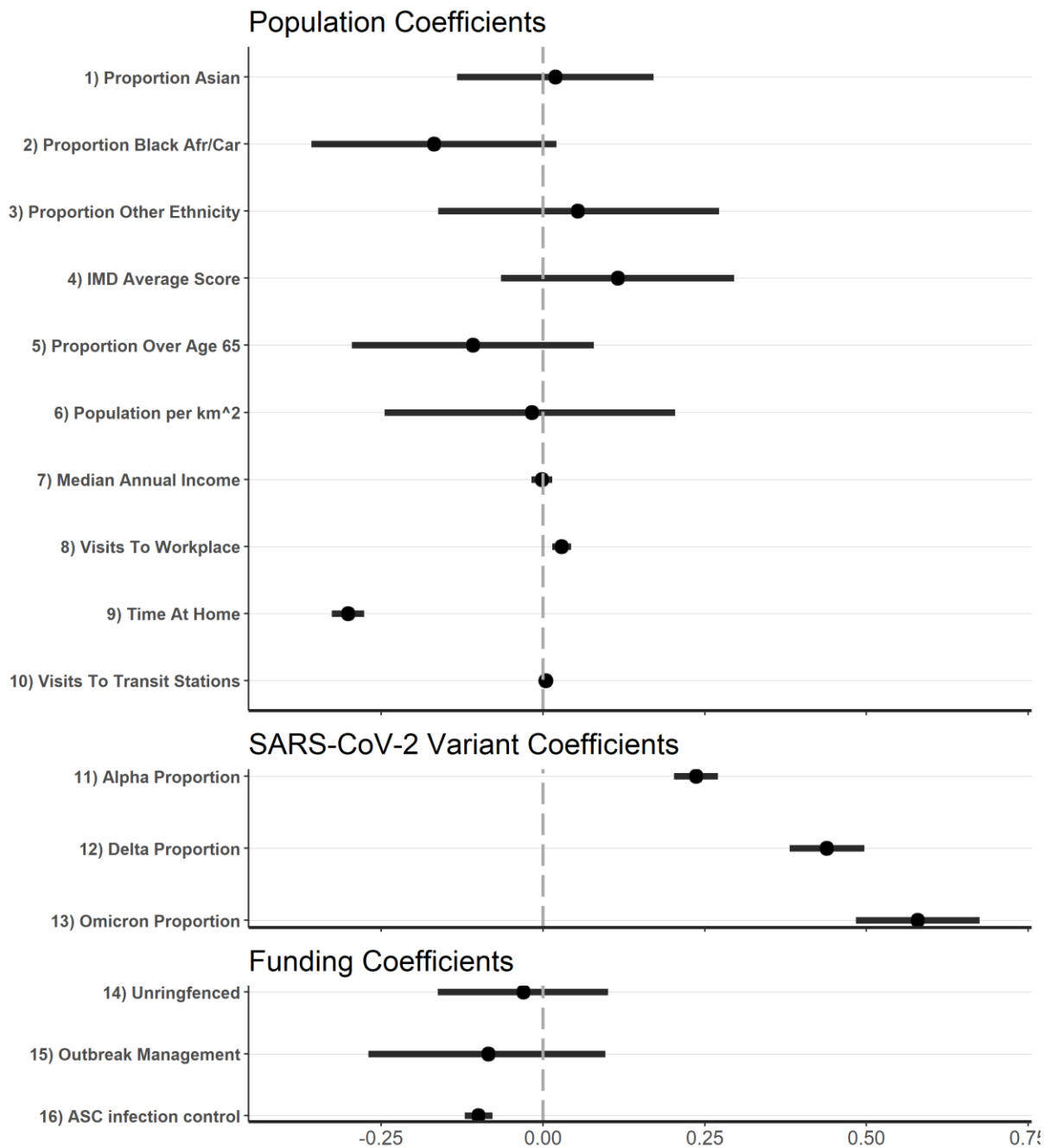
Figure 3: Posterior estimates of all covariate coefficients (parameter \beta ). These values are separated into three categories: those capturing population effects, those capturing variants-of-concern, and those capturing funding allocations. Black dots represent the mean estimate, black lines the 95% CrI. The dashed grey line marks 0. A positive value indicates that the effective reproduction number increases with higher values of the associated covariate, a negative value indicates that the effective reproduction number decreases with higher values of the associated covariate.
