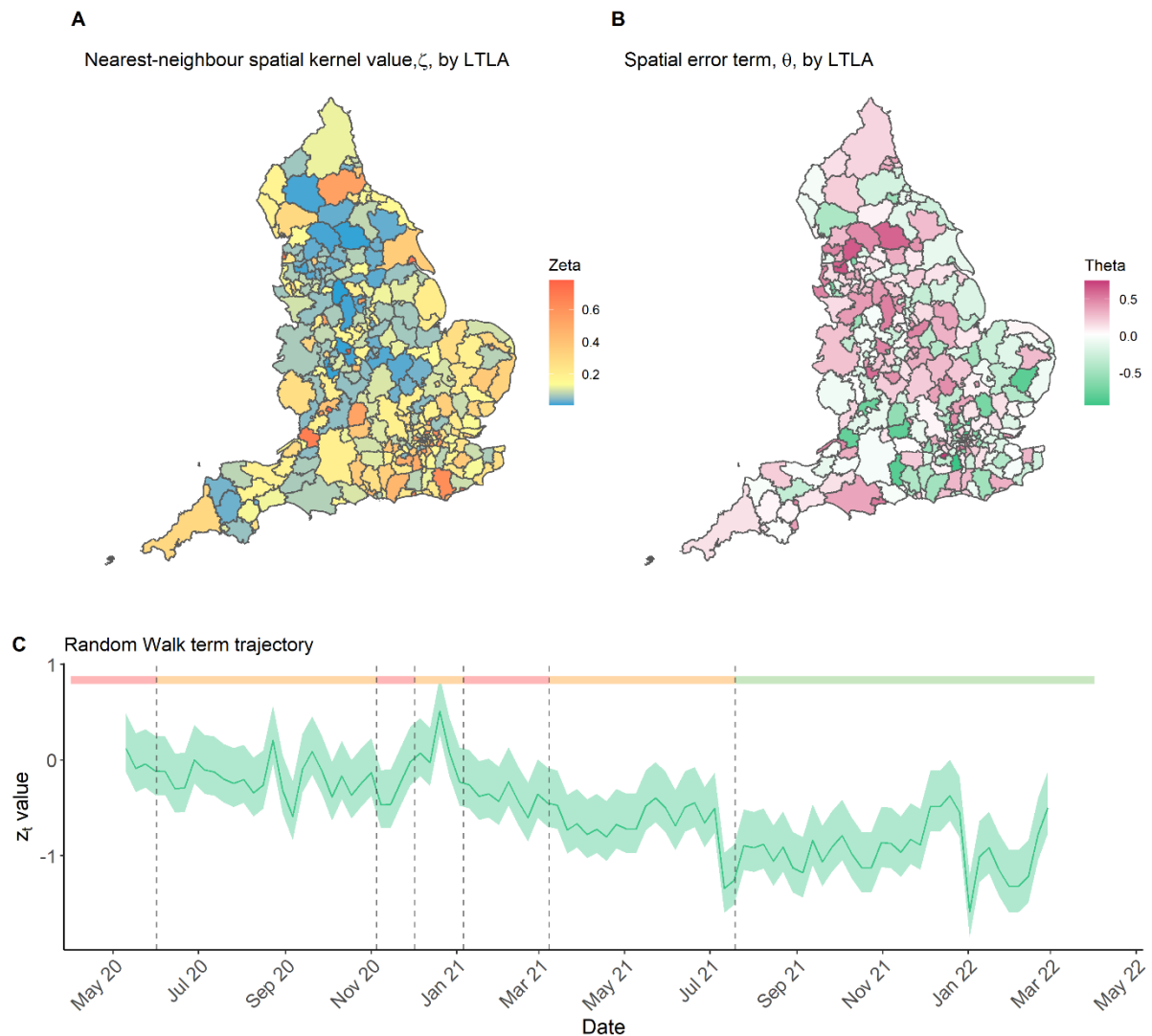
190 Figure 4: Model variables contributing to the LTLA-varying and week-varying effective reproduction number. (A) 191 Estimates of the LTLA-varying parameter \zeta_i , denoting what proportion of the cases in adjacent LTLAs cause 192 secondary cases in LTLA i the following week. (B) The remaining spatial error term, \theta_i , capturing underlying 193 differences in LTLA reproduction numbers not explained by the sixteen considered covariates ( x_{i,t-1} \beta ). 194 The random walk term applied to all LTLAs capturing a baseline time-varying change to the reproduction number. 195 Solid line shows the mean estimate and the shaded region the 95% CrI. Dashed lines and shaded bar at the top 196 of the plot again mark areas of full (red), partial (orange) and no (green) stay-at-home orders. Boundary source: 197 Office for National Statistics licensed under the Open Government Licence v.3.0 29 . Contains OS data © Crown 198 copyright and database right [2024].
