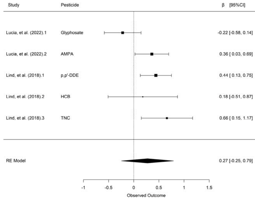
Fig. 2. Forest plot for meta-analysis of associations between pesticide exposure (ln-transformed) and Hannum epigenetic age
