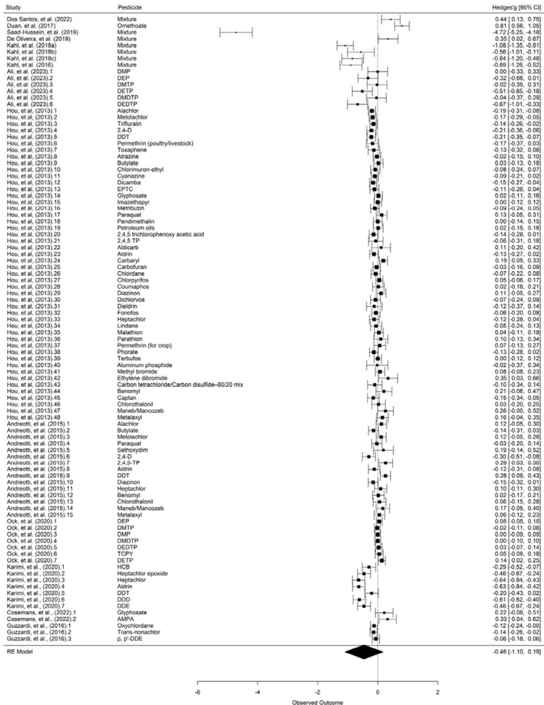
Fig. 3. Forest plot for meta-analysis of associations between pesticide exposure and telomere length
