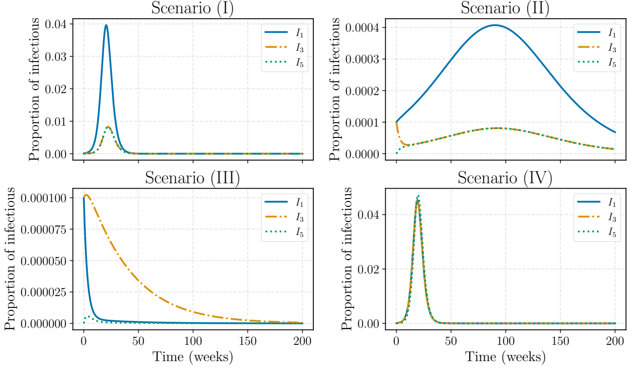
Figure 9: Infectious curves for different scenarios of \beta .
