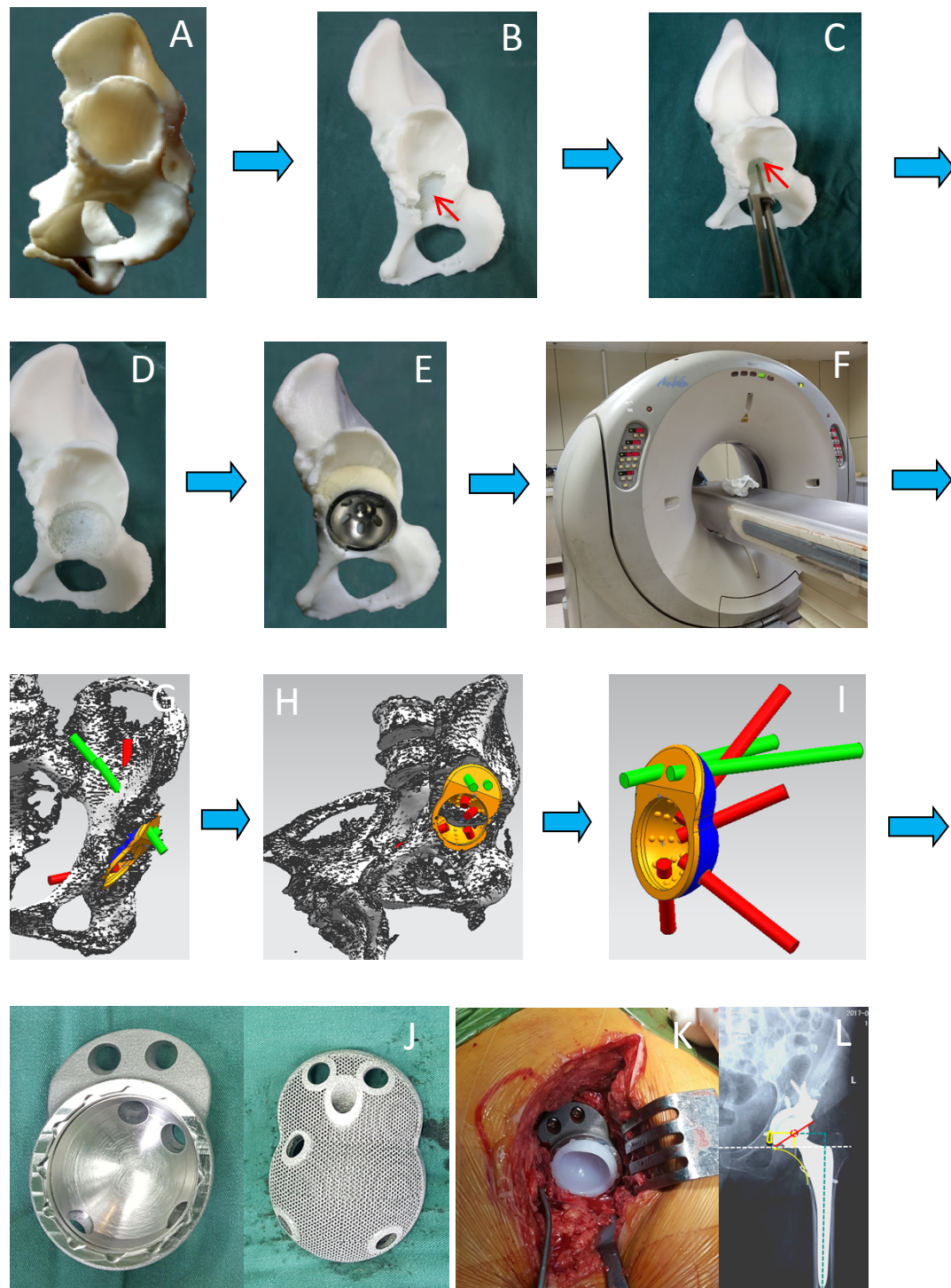
Figure 1 . The flowchart of developing 3D printing integral customized acetabular prosthesis by model method. (A) :3D printing model. (B):Restoring Harris fossa. (C):Locating the acetabular center by ACL.(D):Reaming the acetabulum.(E):Installing the acetabular cup and filling the bone defect with bone wax/cement.(F):CT scan to obtain the data of the cup and bone defect.(G-I):Designing the integral customized acetabular prosthesis.(J):3D printing integral
