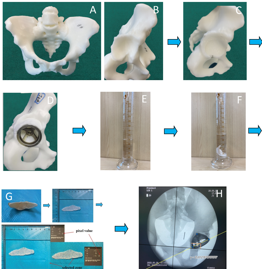
Figure 3. The research process of developing 3D printing integral customized acetabular prosthesis by the model method. (A) : 3D printing the pelvis model using PLA material. (B): the shell-like acetabulum and triangle acetabular fossa. (C) : Reaming the acetabulum.(D):Installing the acetabular test cup and filling the bone defect with bone wax. (E-F): Measuring the volum of bone defect .(G):Measuring surface area of bone defect.(H): Measuring the horizontal and vertical distance of hip center and the anteversion and inclination of acetabular cup on pelvis X-ray. PLA= Polylactic acid.
