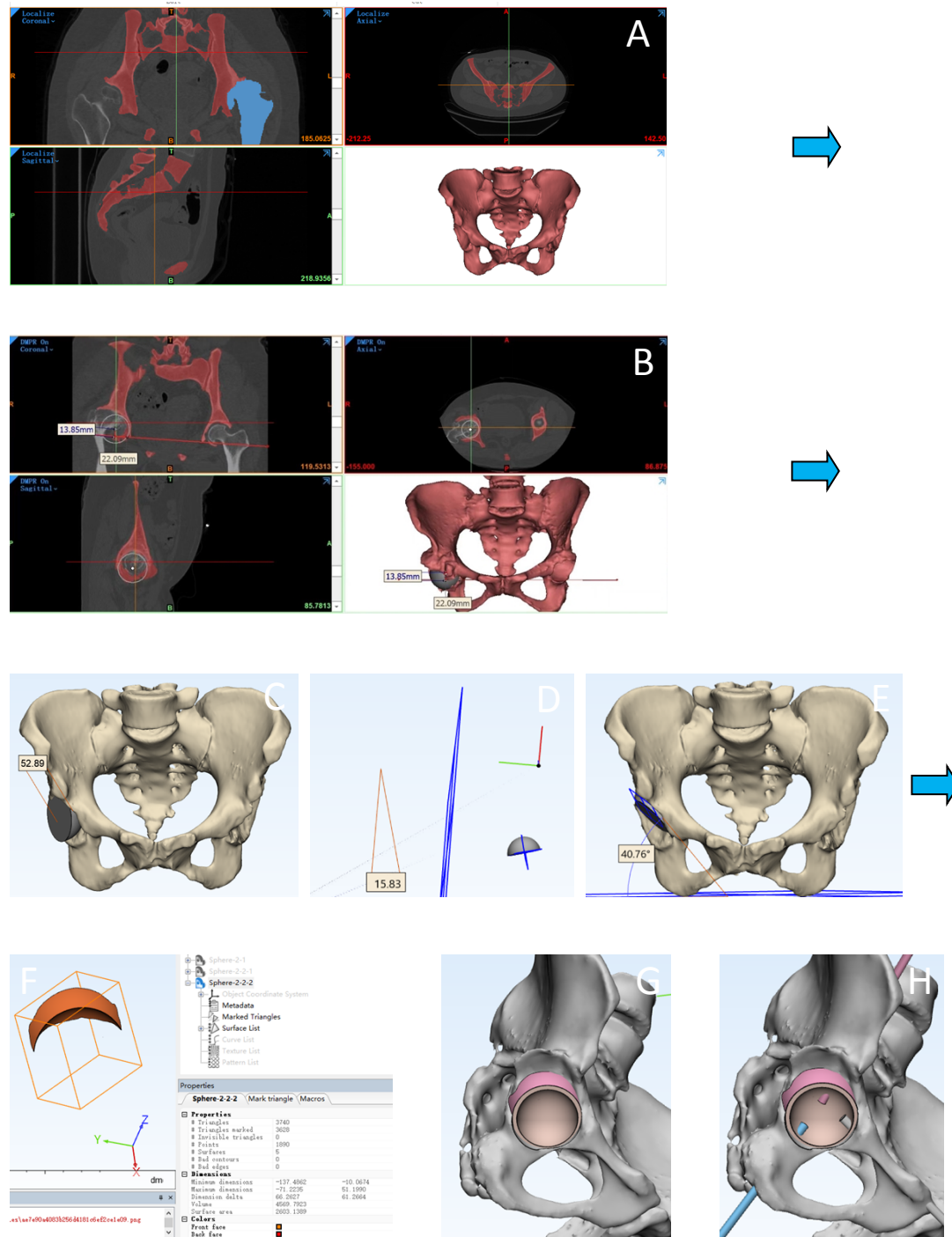
Figure 2. The research process of developing 3D printing integral customized acetabular prosthesis by the software method. (A) :Reconstructing the pelvis model by Mimics software.(B):Restoring hip center and measuring the horizontal and vertical distance by Mimics software .(C-E): Setting the anteversion and inclination of acetabular prosthesis by 3-Matic software .(F):Measuring the volum and surface area of the wing part of acetabular prosthesis(bone defect) by 3-Matic software.(G,H):Installing the integral customized acetabular
