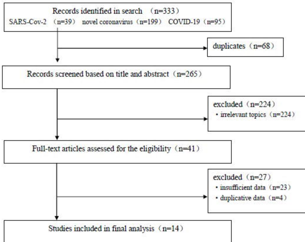
Flowchart diagram of selected studies included in this meta-analysis
