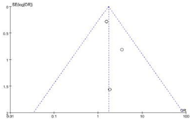
Funnel plot of Fever
