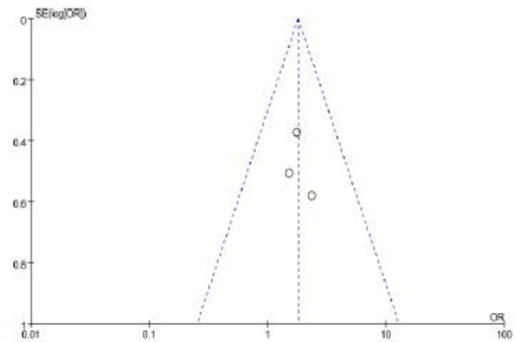
Funnel plot of Diarrhea
