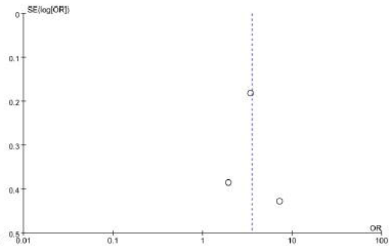
Funnel plot of Polypnea/dyspnea
