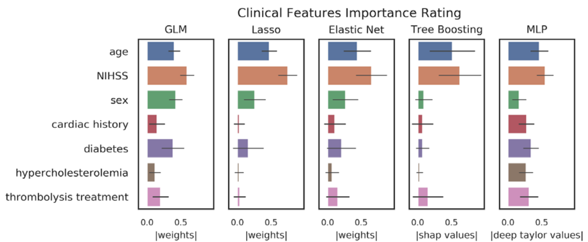
Fig 3. Graphical representation of the feature importance. The figure illustrates the features rating derived from the model-tailored interpretability methods for generalized linear model (GLM), Lasso, Elastic net, Catboost and multilayer perceptron (MLP). For logistic regression techniques the results are given in weights, for Catboost in Shap(ley) values and for MLP in deep Taylor values that were normalized to the range [0,1]. The bar heights represent means and error bars represent standard deviation over samples (shuffles).
